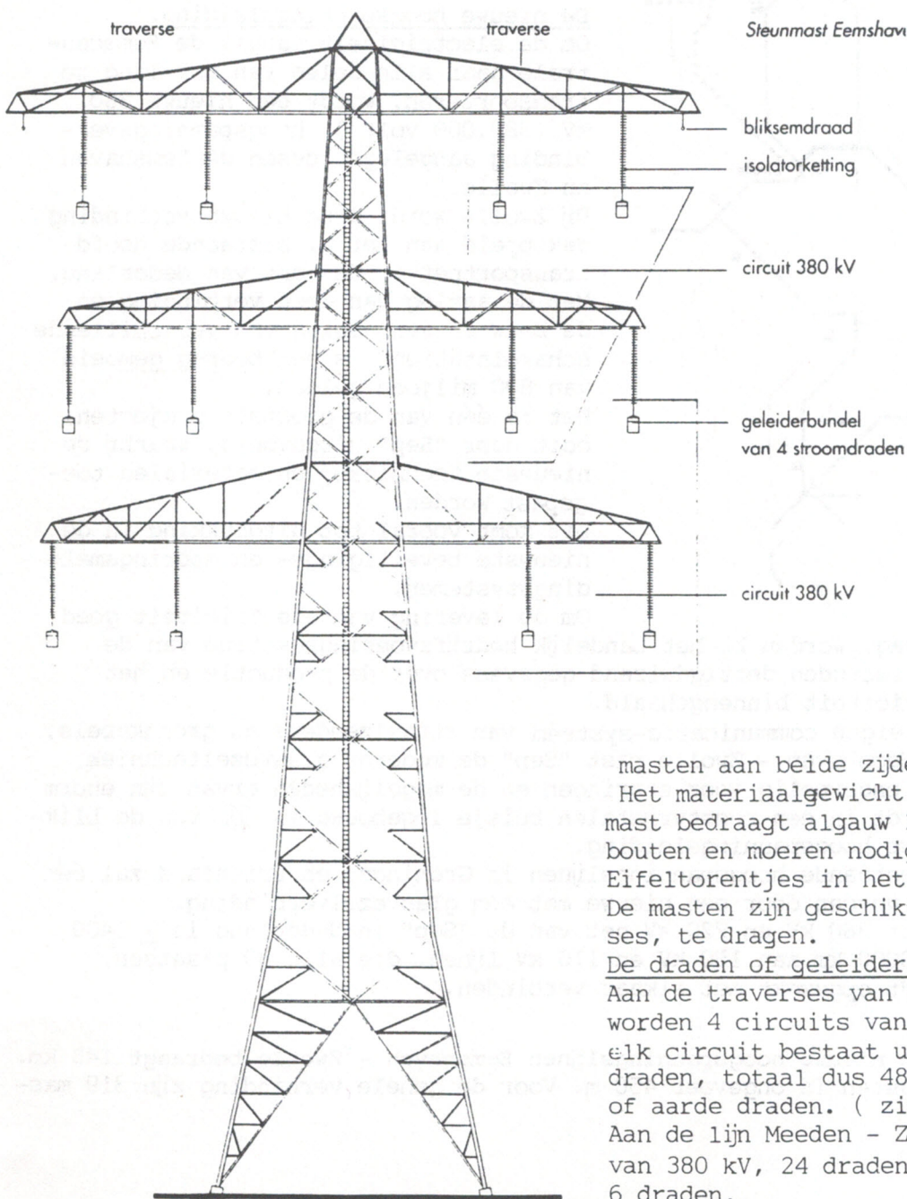
steunmast Eemshaven-Meeden
